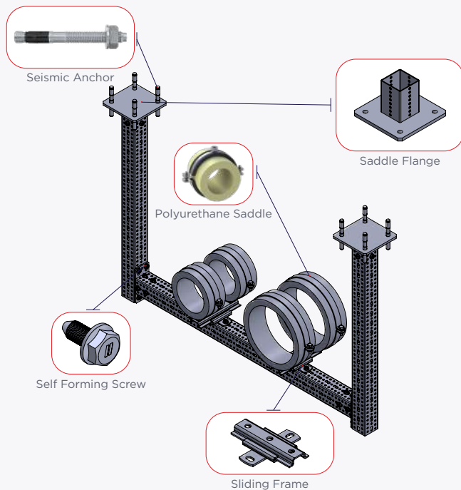
Atlas Ceiling Type Pipe Support
