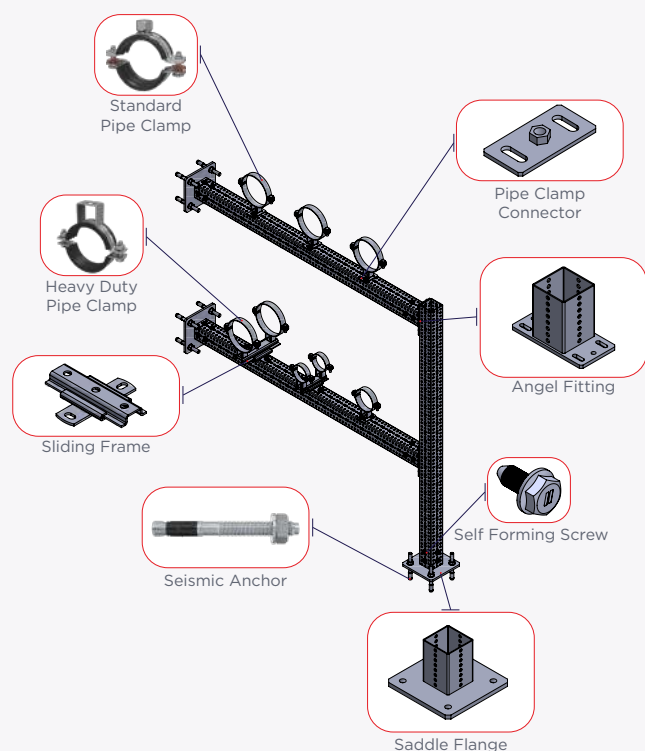
Atlas Floor & Wall Type Pipe Support
