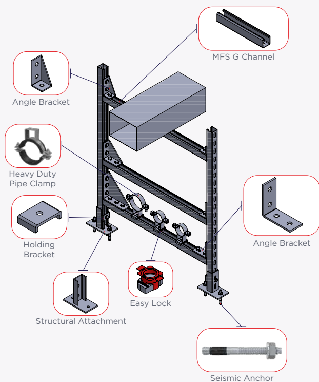
Floor Mounted Support
