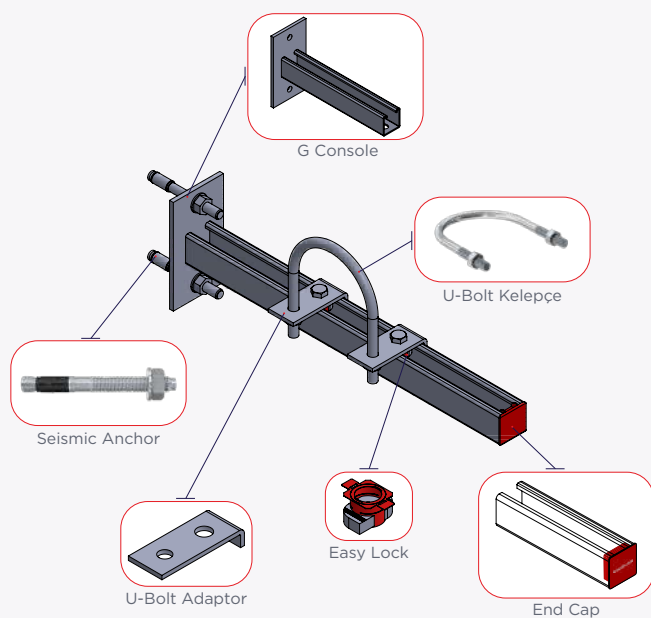
Wall Mounted Console
