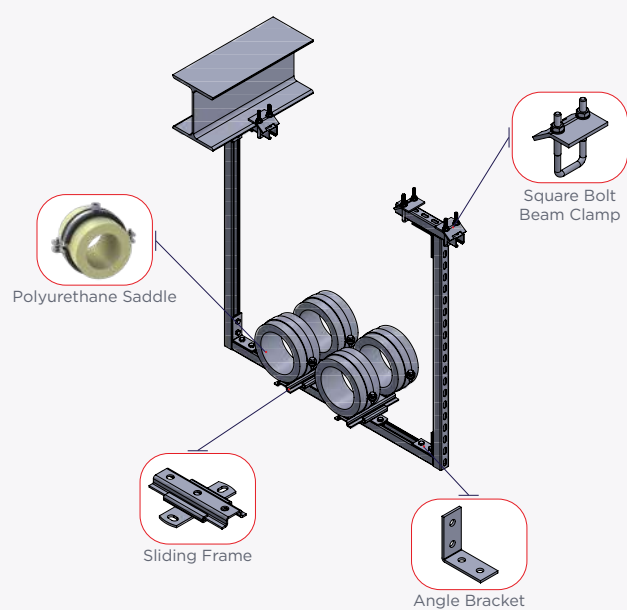
Steel Roof Pipe Support
