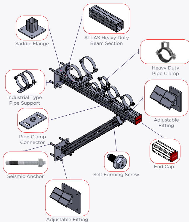
Atlas Wall Mounted Console
