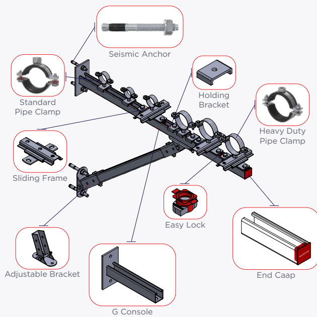
Wall Mounted Console
