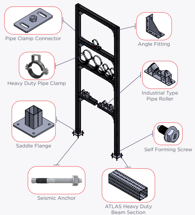
Atlas Floor & Ceiling Type Pipe Support
